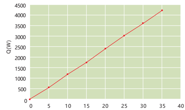
TAP120/TAP120P Δ T(K)
